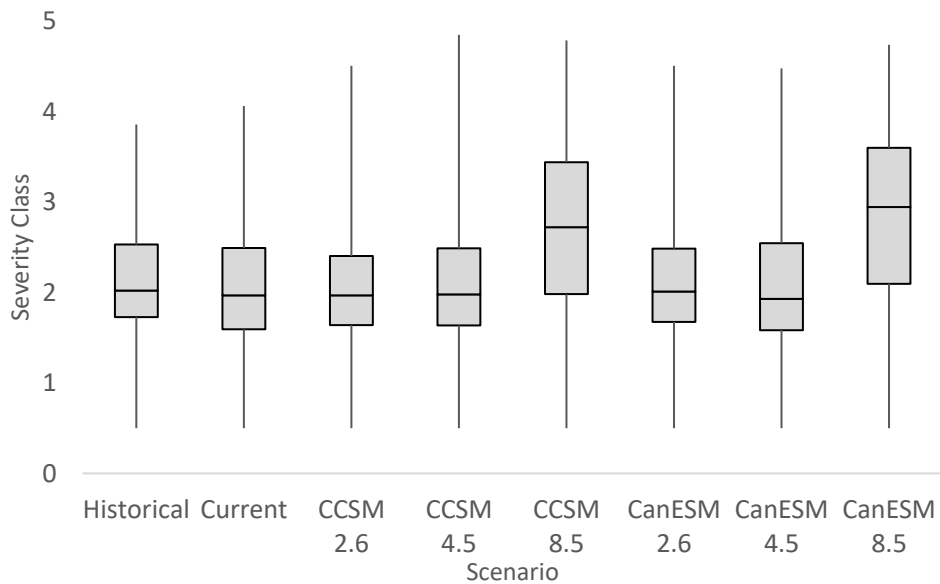
Figure 15. Median, maximum, and minimum severity of fires in each climate scenario. Fire severity was more variable in projected climate scenarios than in the historical and current climate scenarios.
